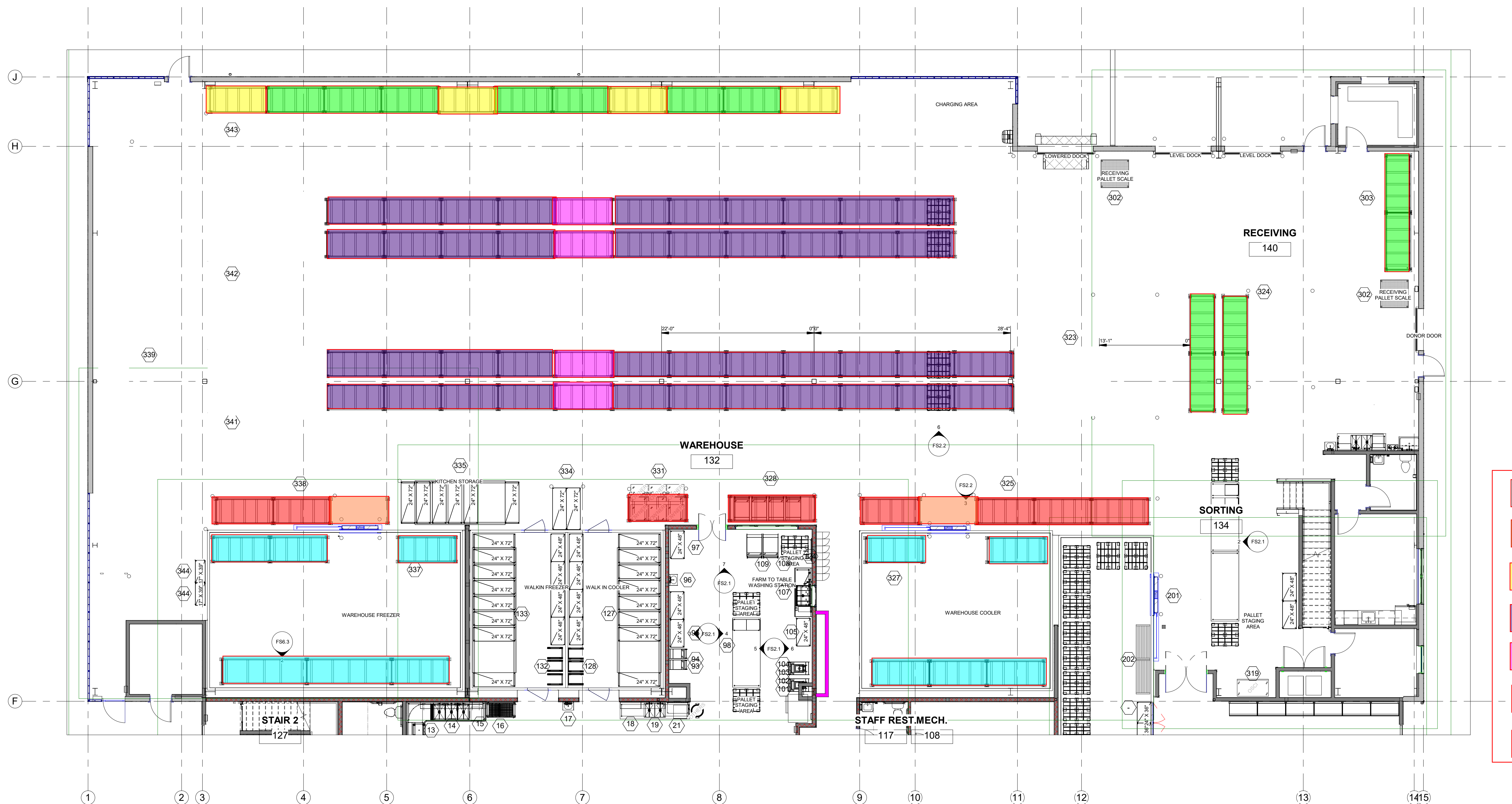
1 EQUIPMENT PLAN - WAREHOUSE SHELVING 1/8" = 1'-0"
